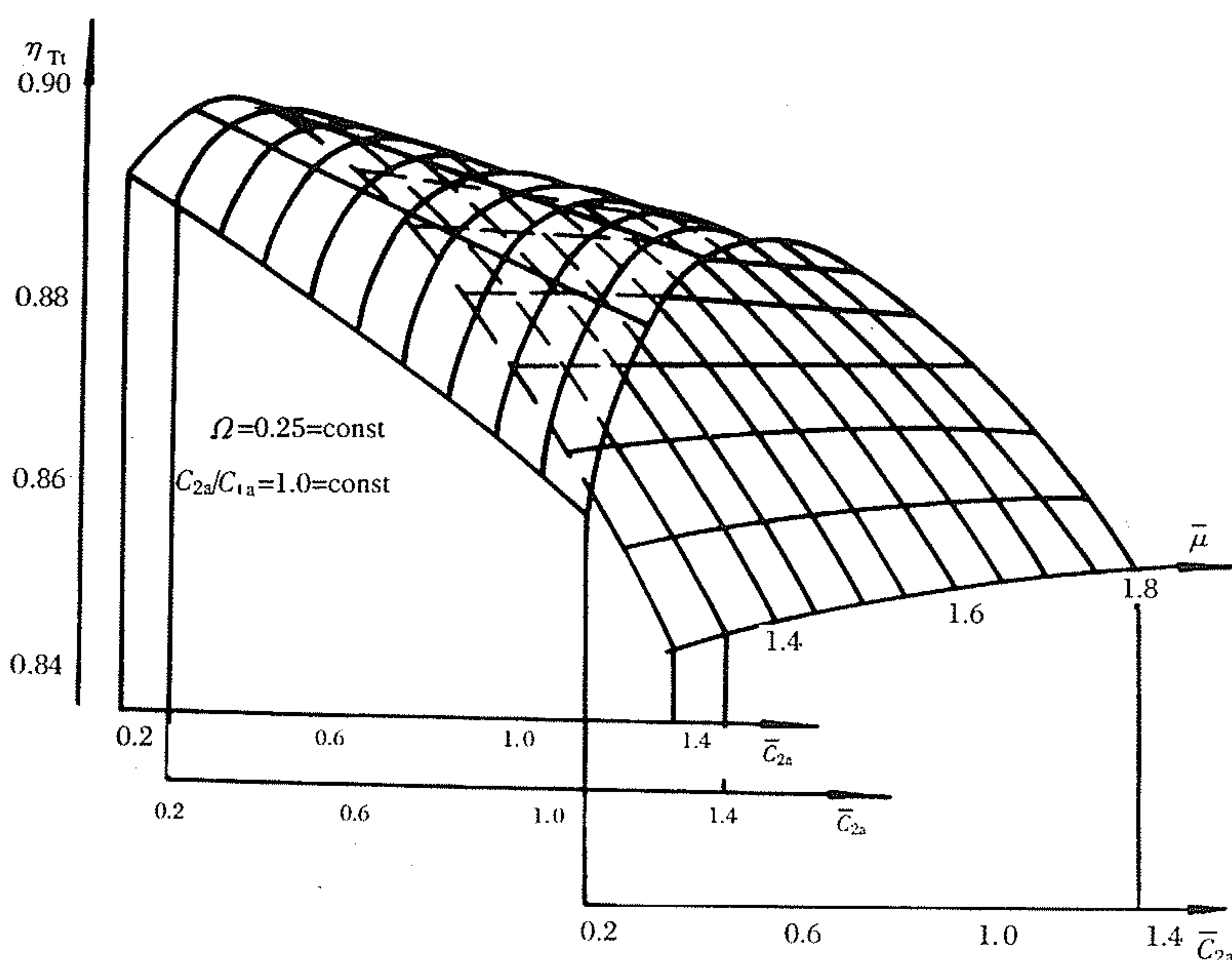
图 2-8 \eta_{Tt} = f(\bar{C}_{2a}, \mu)
