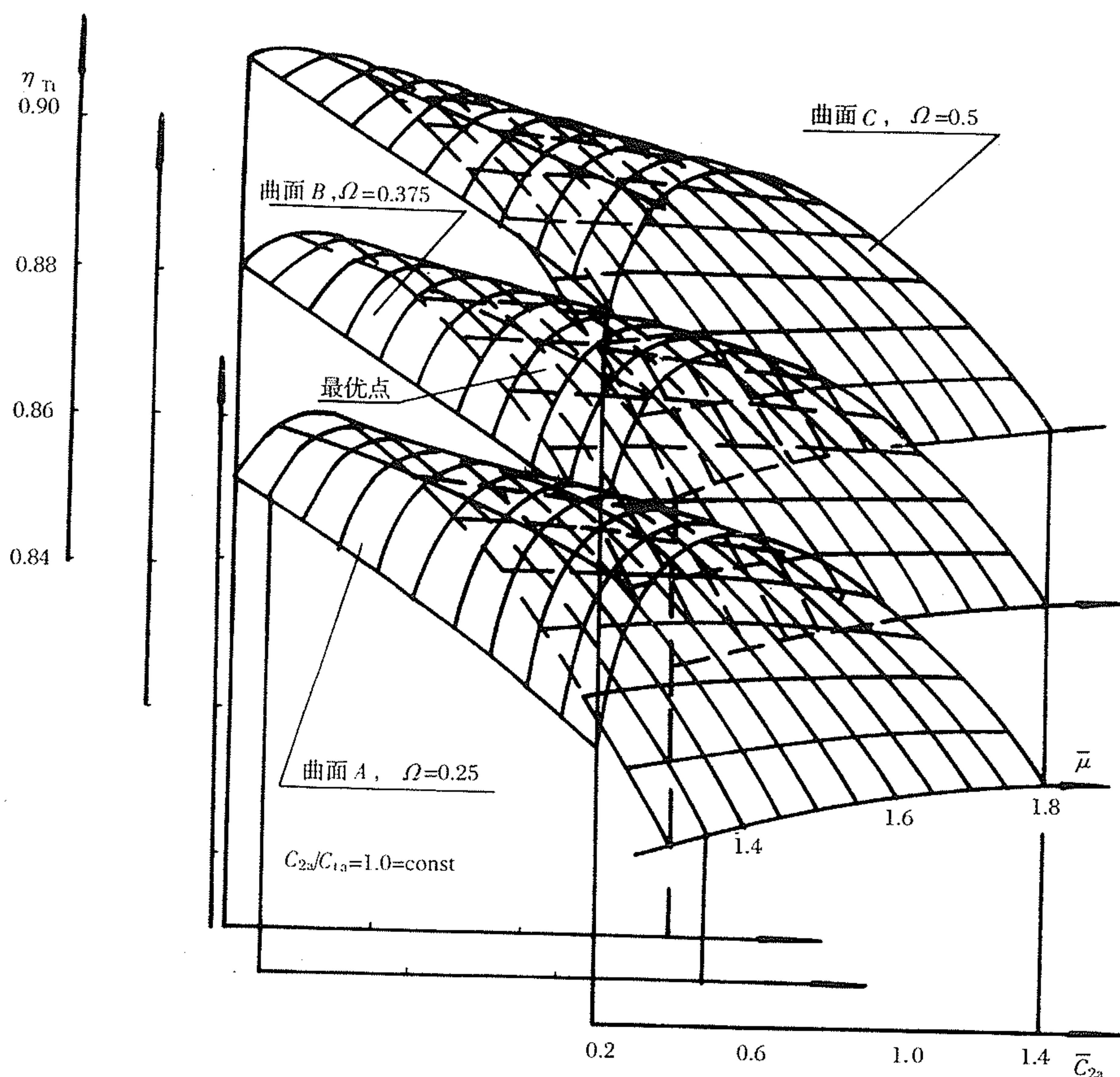
图 2-9 \eta_{Tt} = f(\bar{C}_{2a}, \mu, \Omega)
