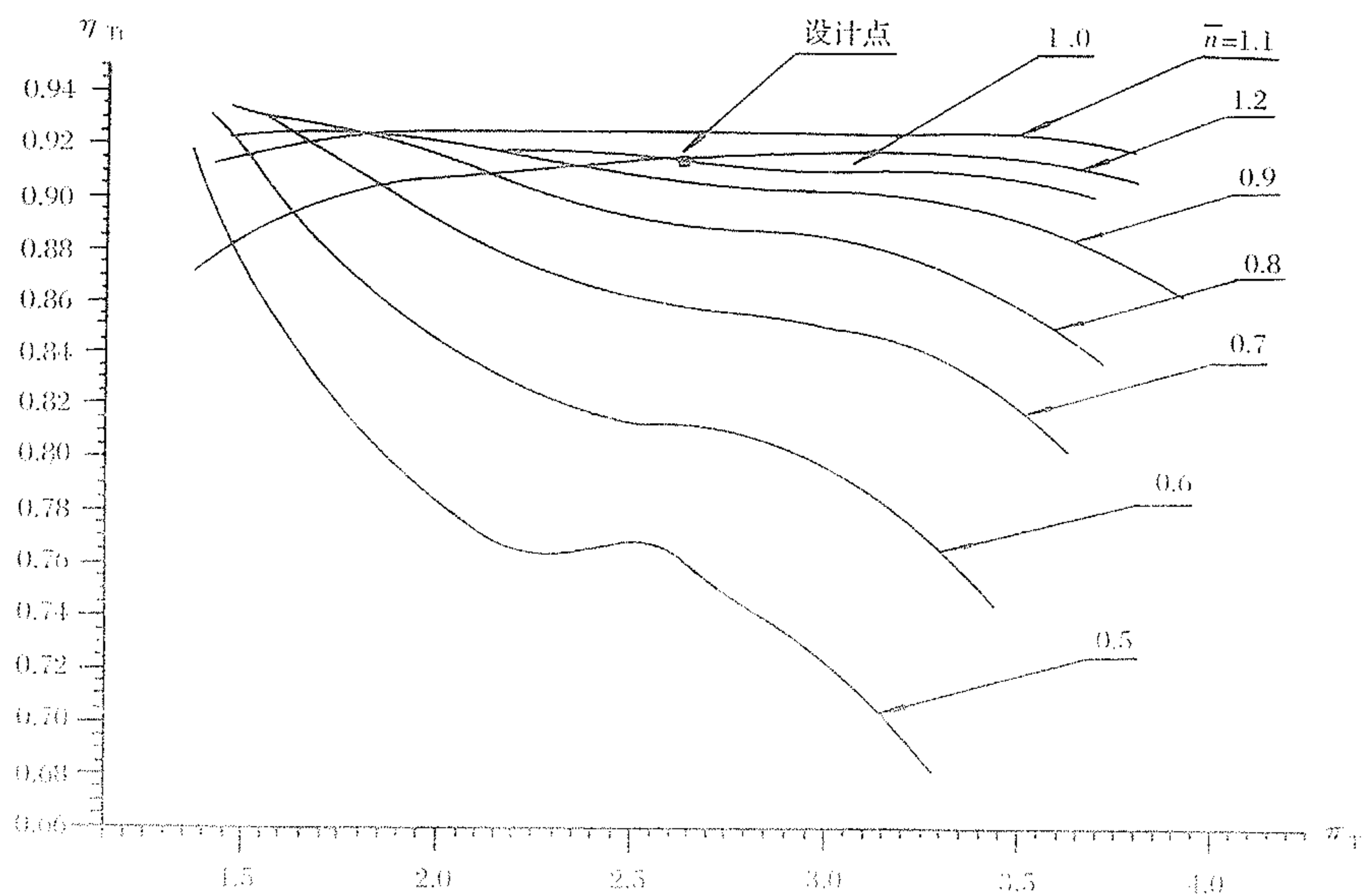
图 13-15 \eta_{T1} = f(\pi_T, \bar{n}) 曲线
