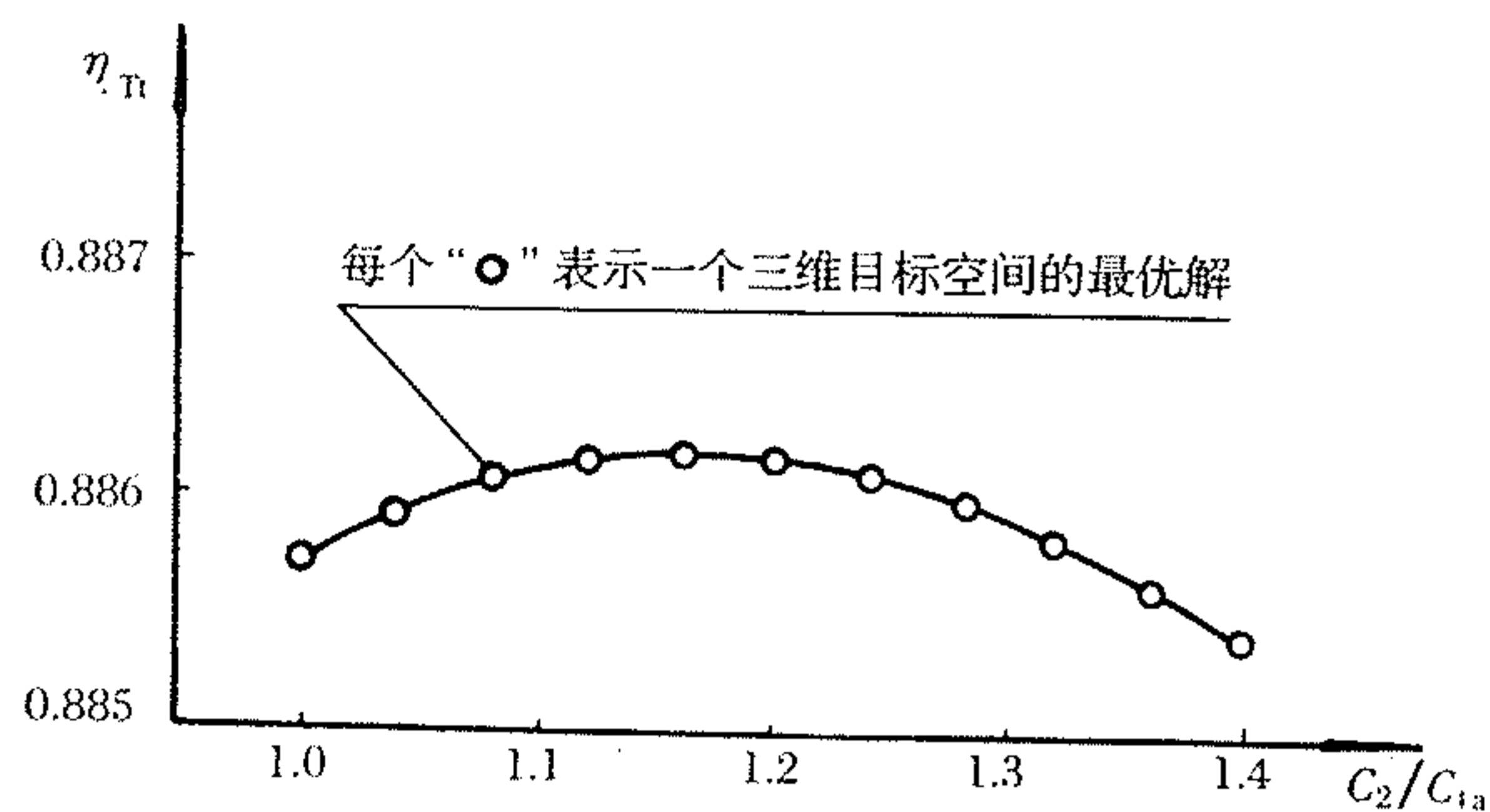
图 2-10 \eta_{Tt} = f(\bar{C}_{2a}, \mu, \Omega, C_{2a}/C_{1a})
