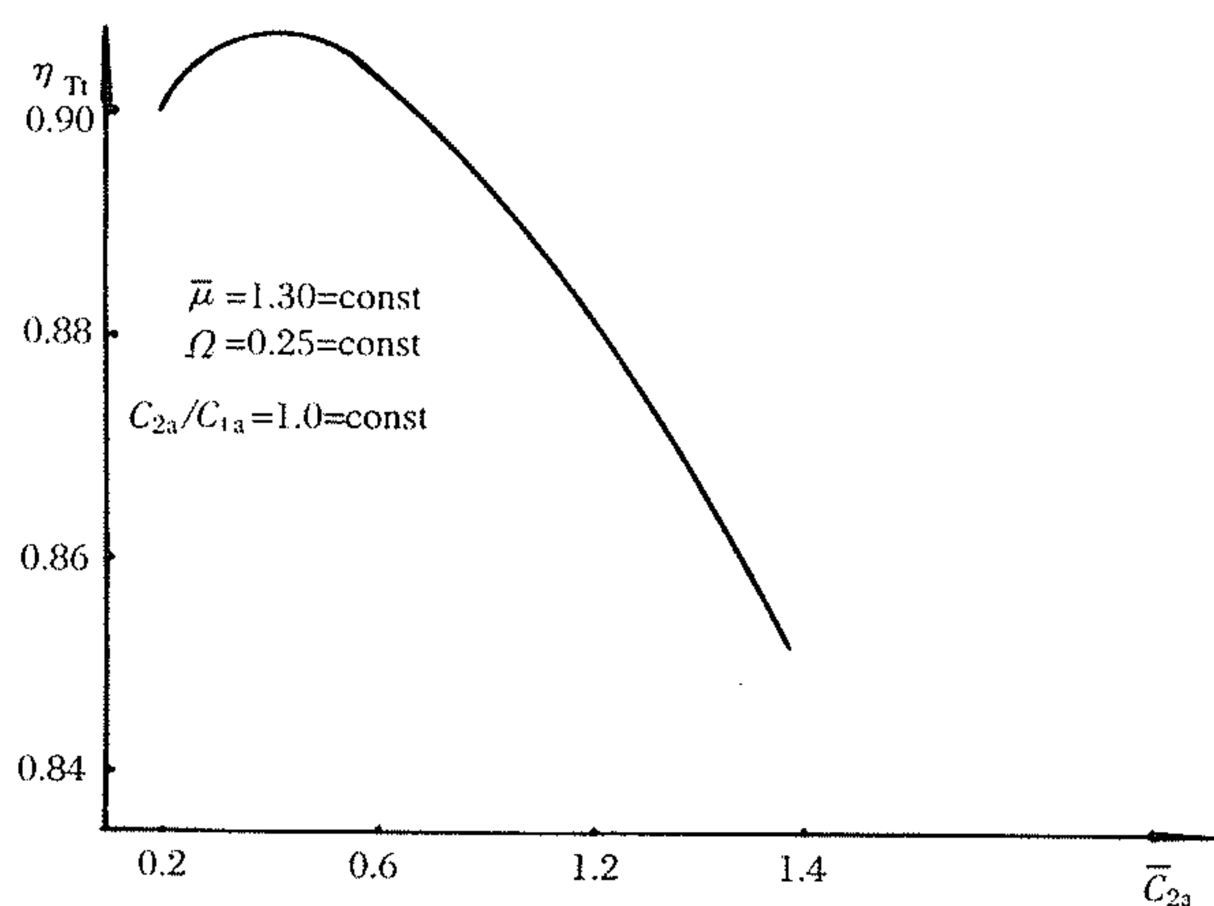
图 2-7 \eta_{Tt} = f(\bar{C}_{2a})
