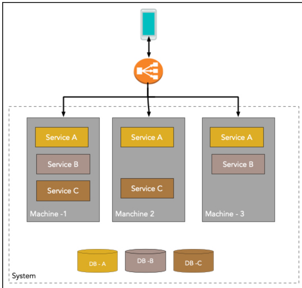
Microservices-based architecture
