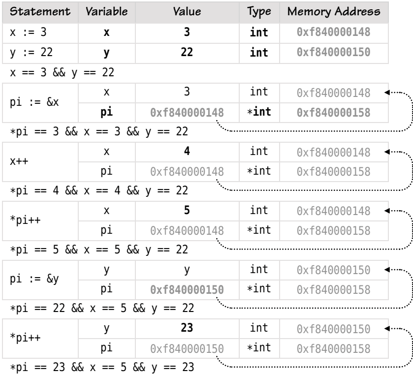
Figure 4.2 Pointers and values
