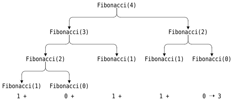
Figure 5.2 Recursive Fibonacci
