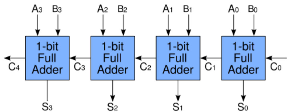
图 14.2. 4-bit Ripple Carry Adder
