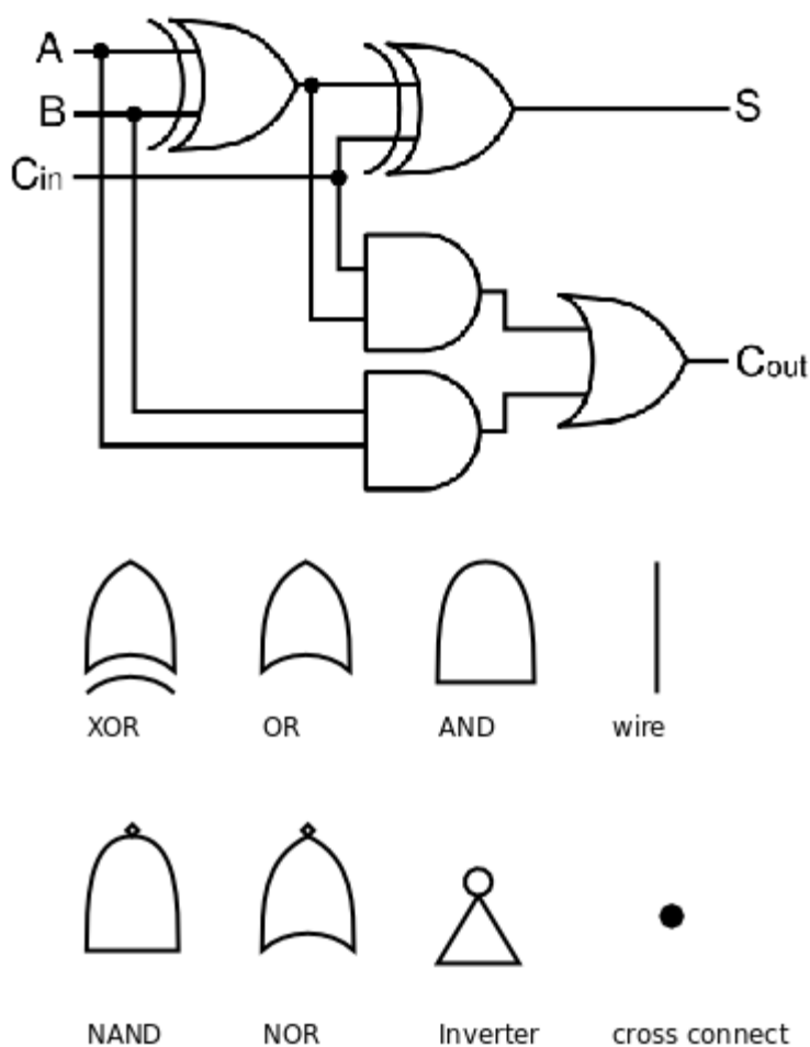
图 14.1. 1-bit Full Adder
