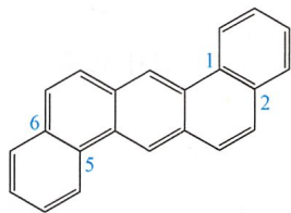
1,2,5,6-二苯并蒽 1,2,5,6-dibenzanthrene
