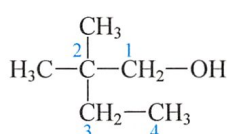
2,2-二甲基丁醇 (2, 2-dimethyl butanol)
