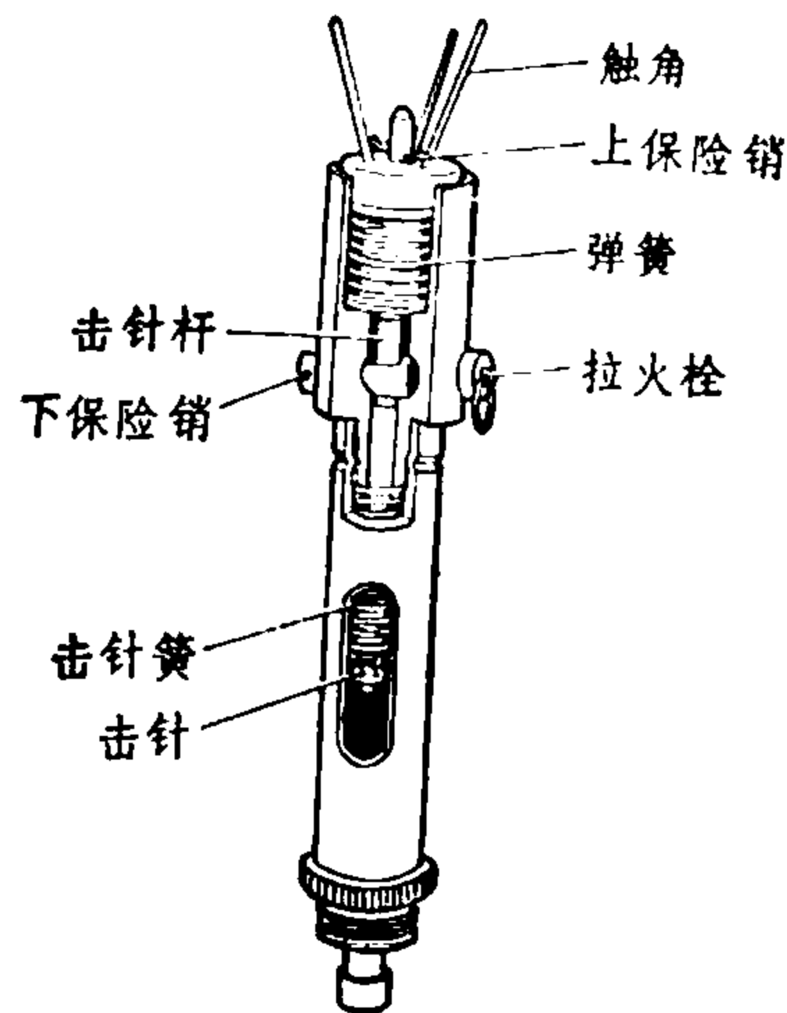
图41 M6A1压、拉两用引信
